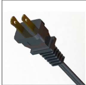
NEMA 1-15P MOP Standard two-prong male plug Cord Shown: 18/2 SPT-2
