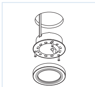
recess mount
