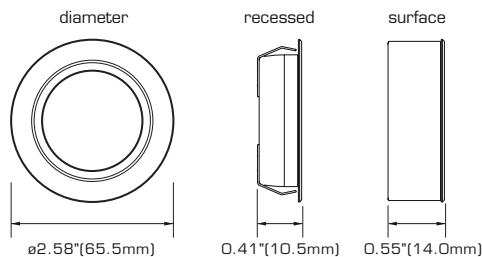
recessed light
