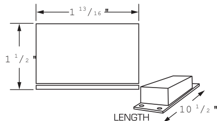
PH8000 cross section
